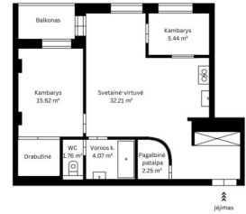
BUTO PLANAS 61.35 m 2
