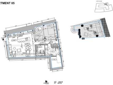
APARTMENT 05
